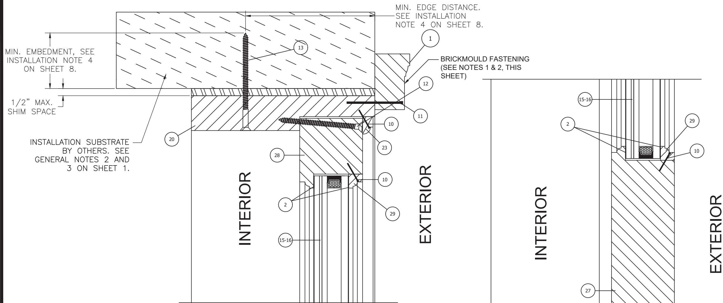
VERTICAL CROSS SECTION TRANSOM HEAD WOOD FRAMING, 2X WOOD BUCK OR CONCRETE/MASONRY SUBSTRATES APPROVED. GLAZED PANEL SHOWN.
