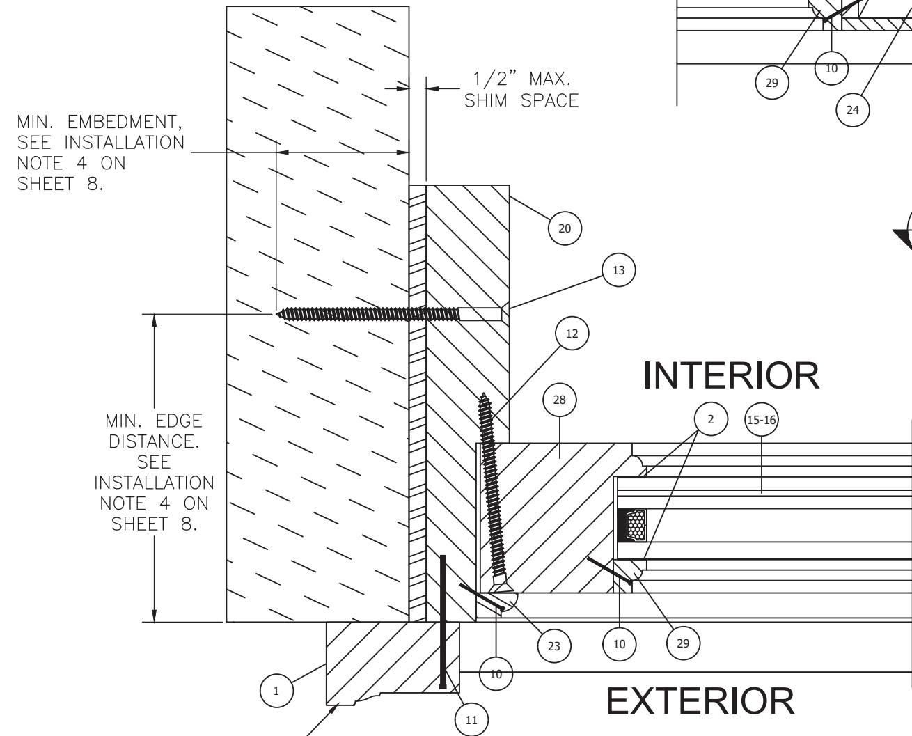
HORIZONTAL CROSS SECTION TRANSOM WOOD FRAMING, 2X WOOD BUCK OR CONCRETE/MASONRY SUBSTRATES APPROVED. GLAZED PANEL SHOWN.
