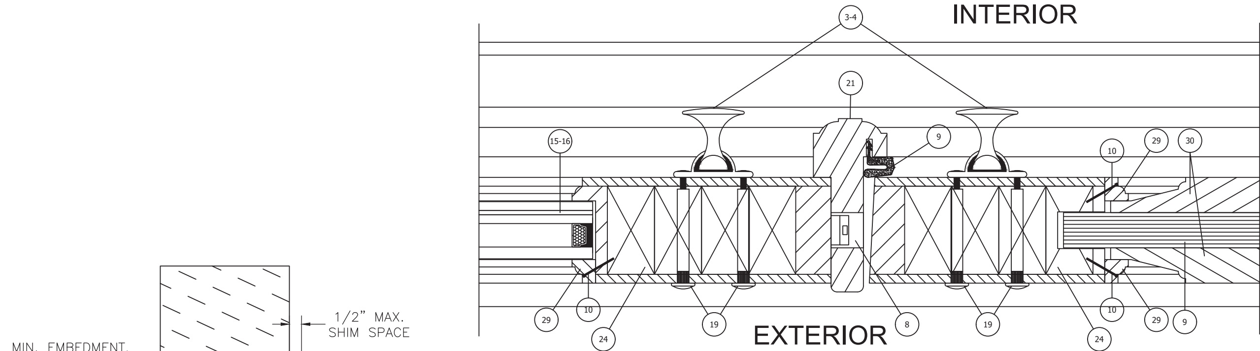
HORIZONTAL CROSS SECTION ASTRAGAL WOOD FRAMING, 2X WOOD BUCK OR CONCRETE/MASONRY SUBSTRATES APPROVED. GLAZED & OPAQUE PANEL SHOWN.
